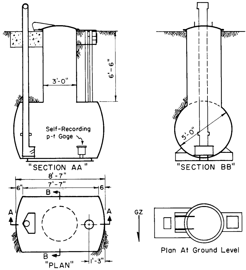
Fig. 9—Pressure plenum for blast closure valve test.
